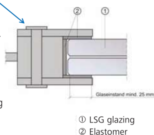
Figure 5: Cross section of edge clamp holder
